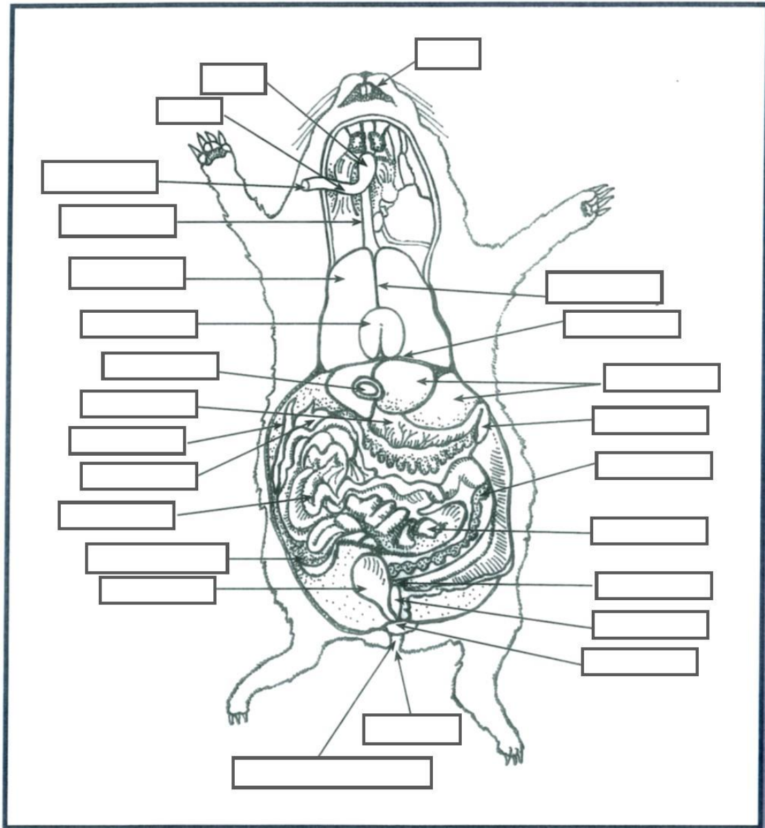
Cavy internal anatomy (female)
